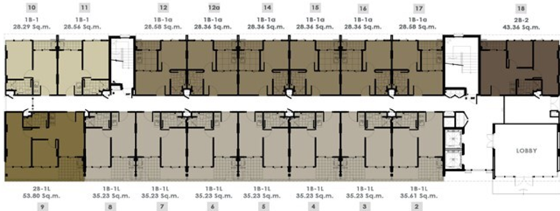
LEVEL 1 FLOORPLAN
